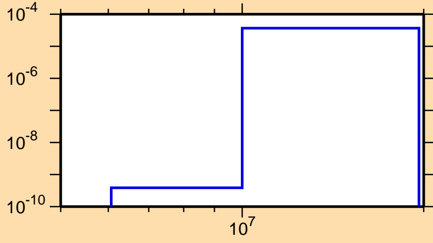
\sigma vs. E for ^{161}\text{Tb}(n,n\alpha)
