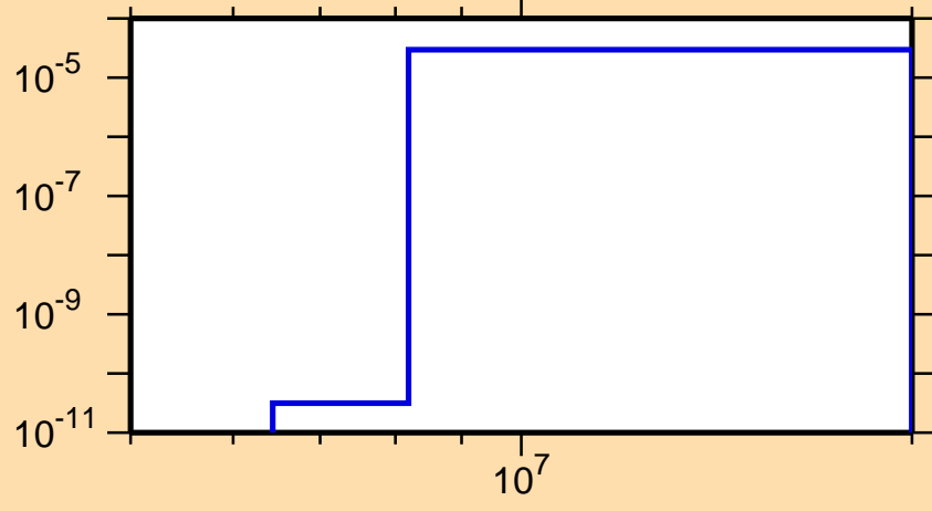
\sigma vs. E for ^{161}\text{Tb}(n,n\alpha)
