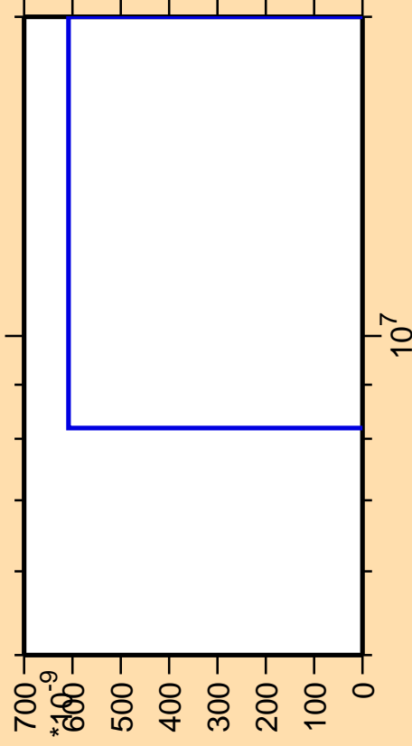
\Delta\sigma/\sigma vs. E for ^{161}\text{Tb}(\text{mt } 11)
