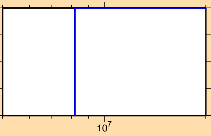
\sigma vs. E for ^{161}\text{Tb}(n,2np)
