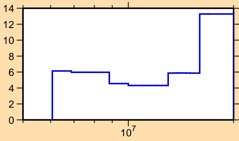
\Delta\sigma/\sigma vs. E for ^{162}\text{Tb}(n,2n)
