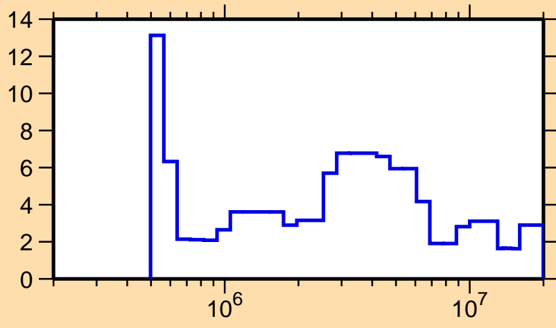
\Delta\sigma/\sigma vs. E for ^{162}\text{Tb}(n,\text{el.})
