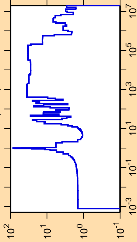
\Delta\sigma/\sigma vs. E for ^{162}\text{Tb}(n,\text{el.})
