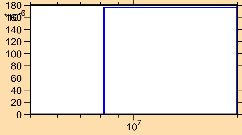
\sigma vs. E for ^{162}\text{Tb}(n,np)
