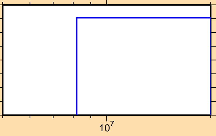
\sigma vs. E for ^{162}\text{Tb}(n,2np)
