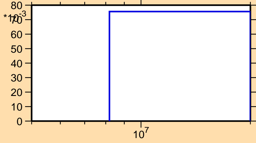
\sigma vs. E for ^{162}\text{Tb}(n,3n)
