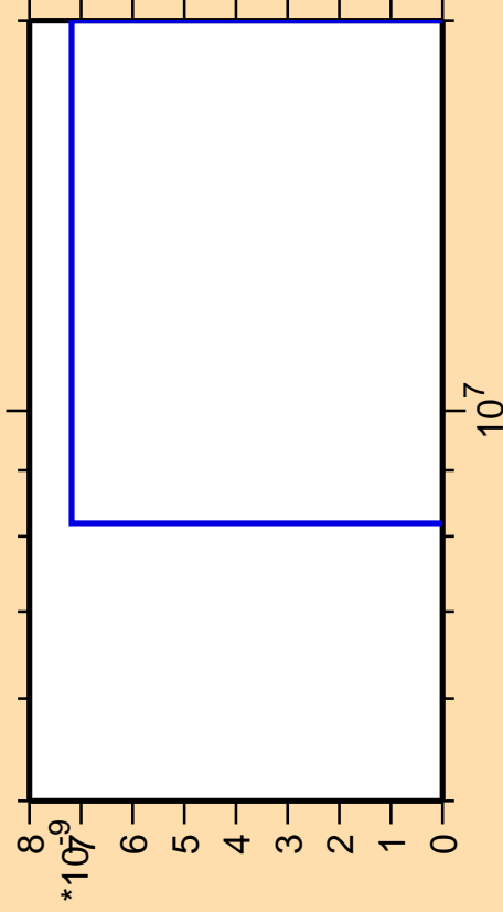
\Delta\sigma/\sigma vs. E for ^{162}\text{Tb}(\text{mt } 11)
