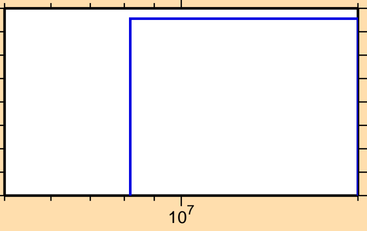
\sigma vs. E for ^{162}\text{Tb}(n,3n)
