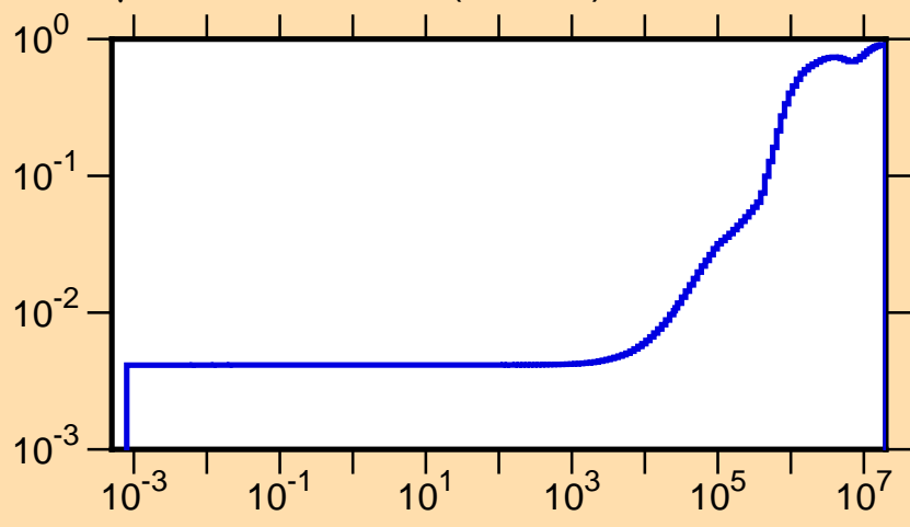
\mu vs. E for ^{163}\text{Tb}(\text{mt251})
