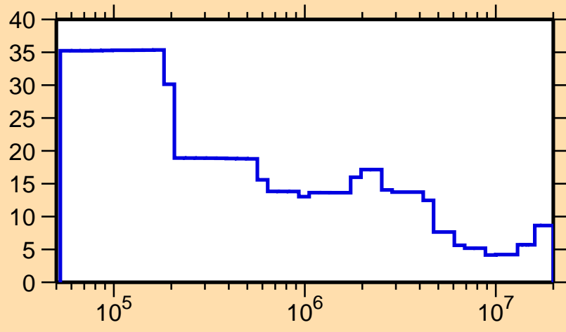
\Delta\sigma/\sigma vs. E for ^{163}\text{Tb}(n,\text{tot.})
