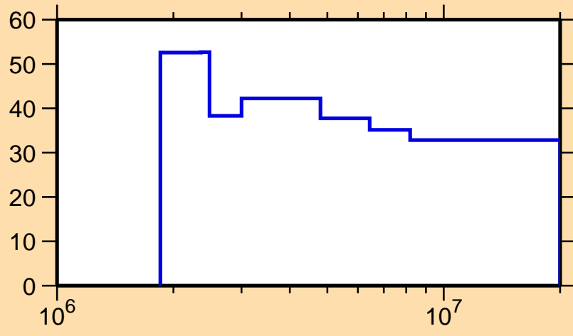
\Delta\sigma/\sigma vs. E for ^{163}\text{Tb}(n,n_1)
