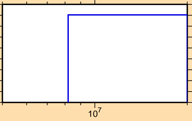
\sigma vs. E for ^{163}\text{Tb}(n,t)
