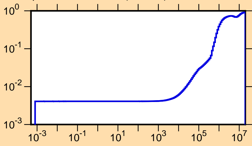
\mu vs. E for ^{165}\text{Tb}(\text{mt251})
