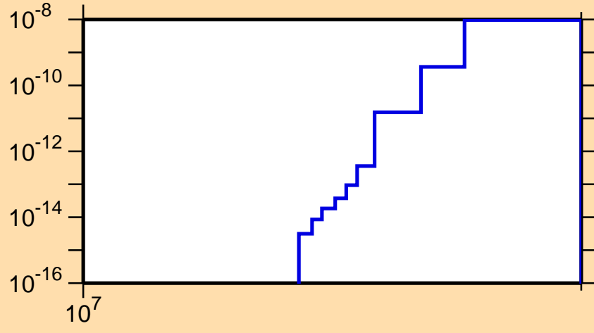
\sigma vs. E for ^{165}\text{Tb}(n,2n\alpha)
