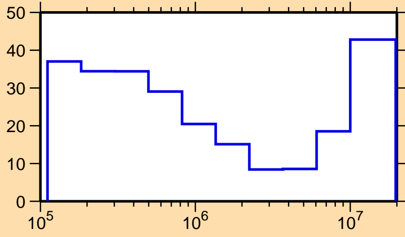
\Delta\sigma/\sigma vs. E for ^{165}\text{Tb}(n,\text{inel.})
