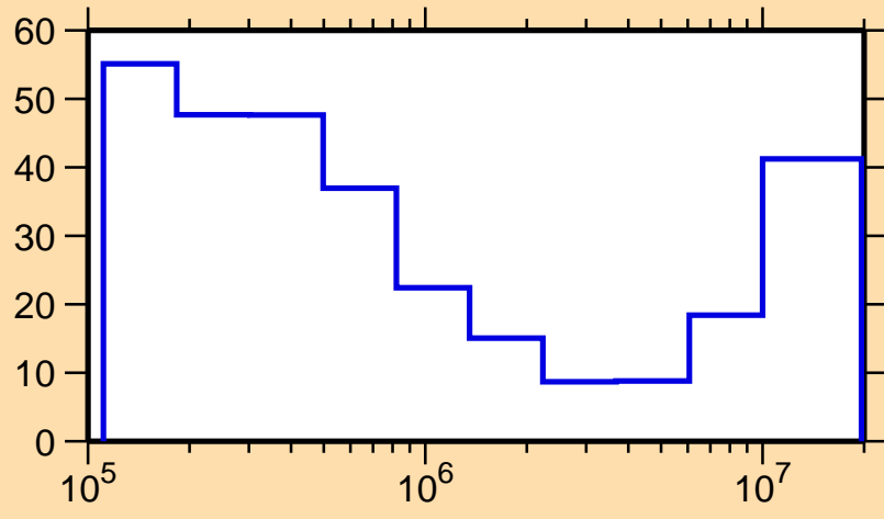
\Delta\sigma/\sigma vs. E for ^{165}\text{Tb}(n,n\text{cont.})
