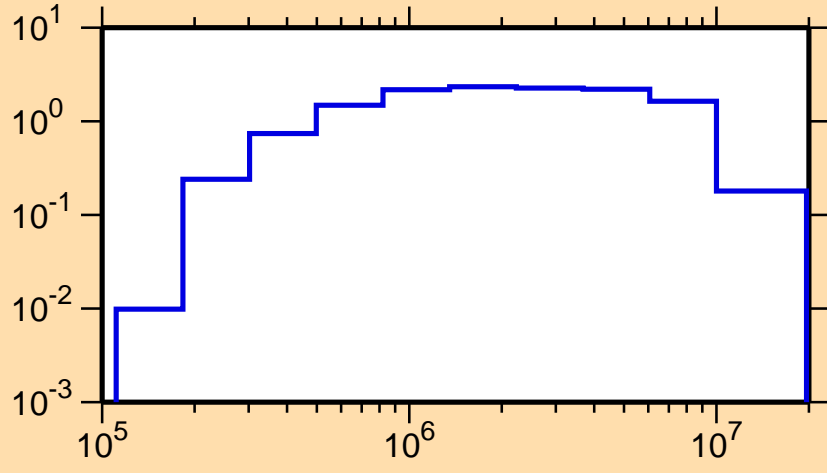
\sigma vs. E for ^{165}\text{Tb}(n,n\text{cont.})
