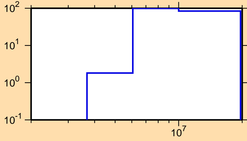
\Delta\sigma/\sigma vs. E for ^{165}\text{Tb}(n,p)
