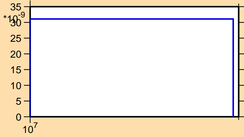
\sigma vs. E for ^{165}\text{Tb}(n,nt)
