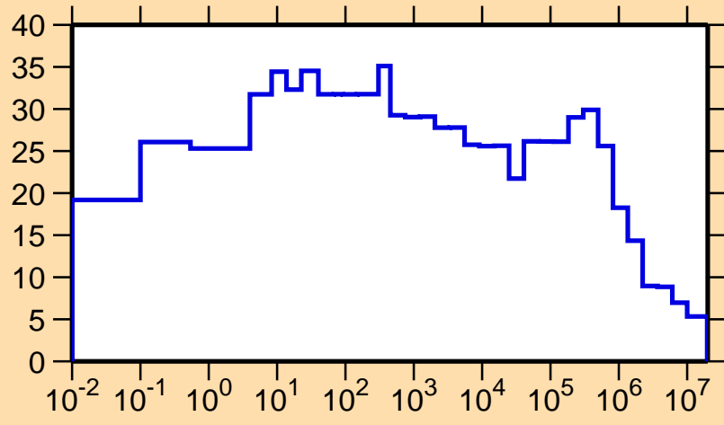
\Delta\sigma/\sigma vs. E for ^{165}\text{Tb}(n,\text{nonel.})
