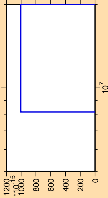
\Delta\sigma/\sigma vs. E for ^{165}\text{Tb} (mt 42)
