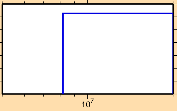
\sigma vs. E for ^{165}\text{Tb}(n,t)
