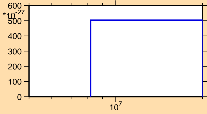
\sigma vs. E for ^{165}\text{Tb} (mt 42)
