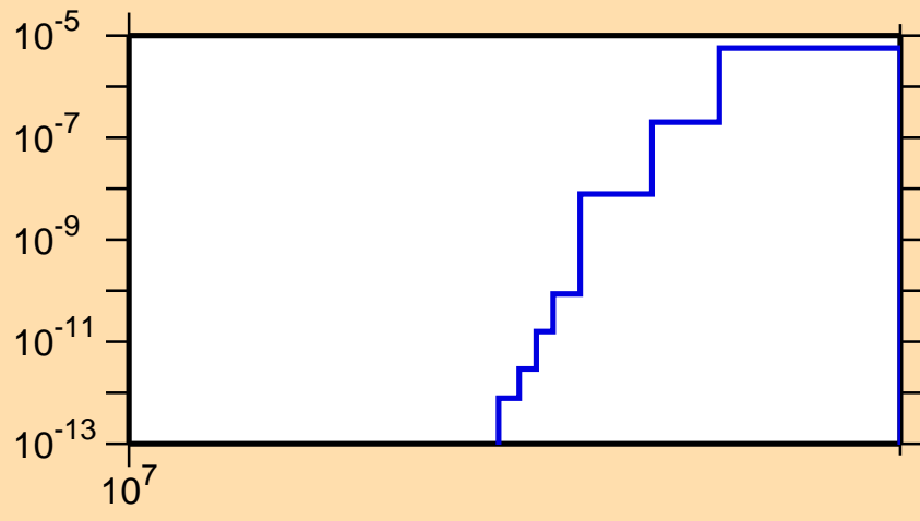
\sigma vs. E for ^{166}\text{Tb}(n,\text{nd})
