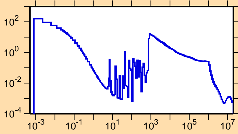
\sigma vs. E for ^{166}\text{Tb}(n,\gamma)
