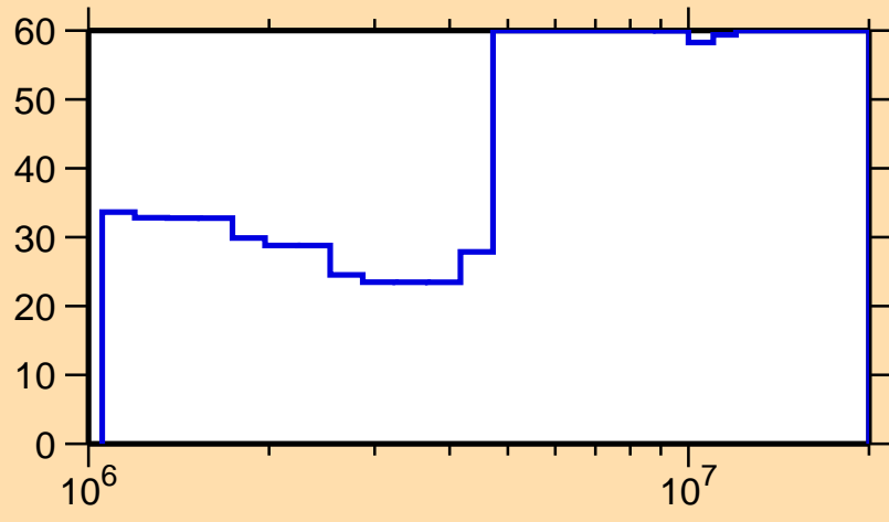
\Delta\sigma/\sigma vs. E for ^{166}\text{Tb}(n,n\text{cont.})
