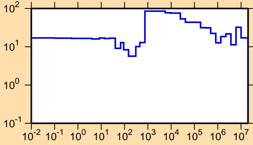
\Delta\sigma/\sigma vs. E for ^{166}\text{Tb}(n,\text{el.})
