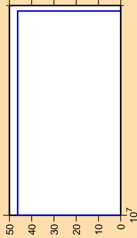
\Delta\sigma/\sigma vs. E for ^{166}\text{Tb}(n,3n)
