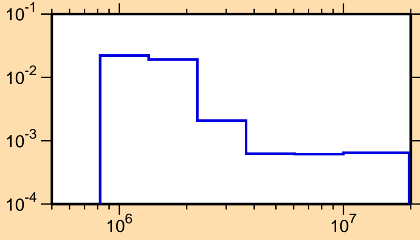
\sigma vs. E for ^{166}\text{Tb}(n,n_4)
