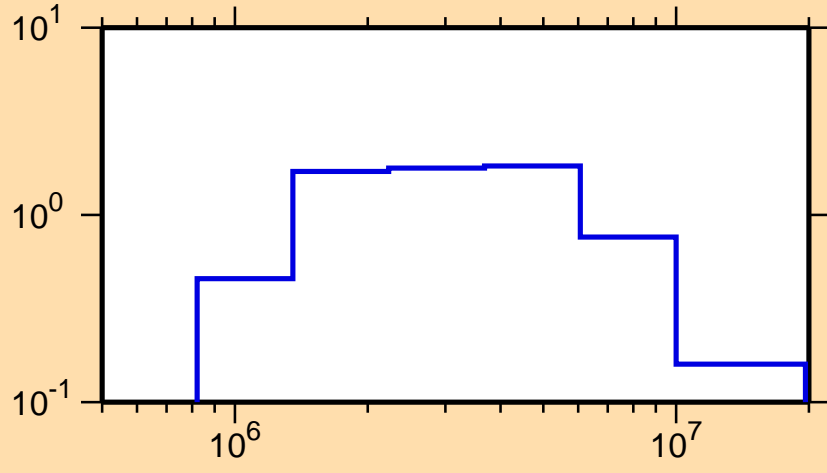
\sigma vs. E for ^{166}\text{Tb}(n,n\text{cont.})
