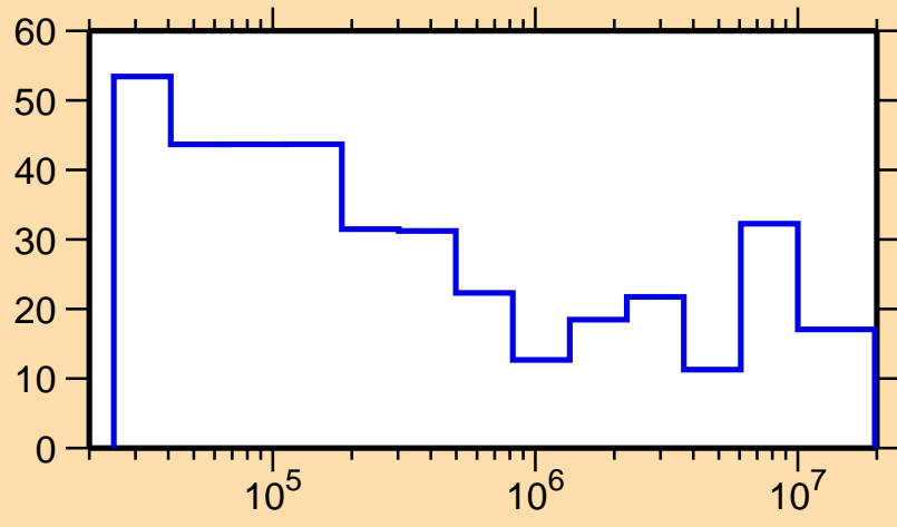
\Delta\sigma/\sigma vs. E for ^{166}\text{Tb}(n,\text{el.})
