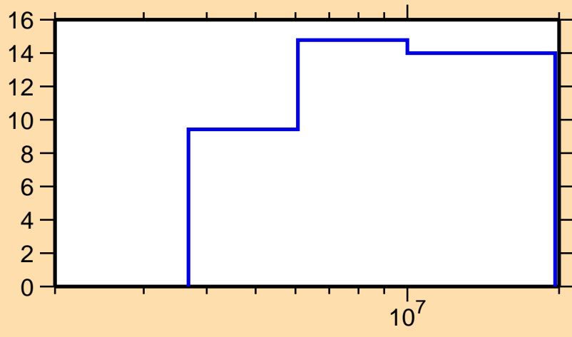
\Delta\sigma/\sigma vs. E for ^{166}\text{Tb}(n,\text{nonel.})
