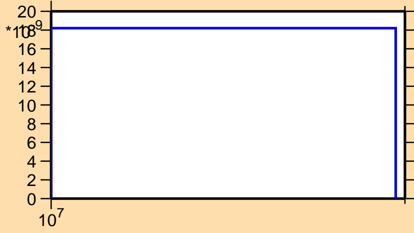
\sigma vs. E for ^{166}\text{Tb}(n,nt)
