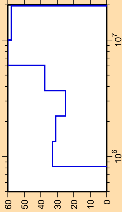
\Delta\sigma/\sigma vs. E for ^{166}\text{Tb}(n,n\text{cont.})
