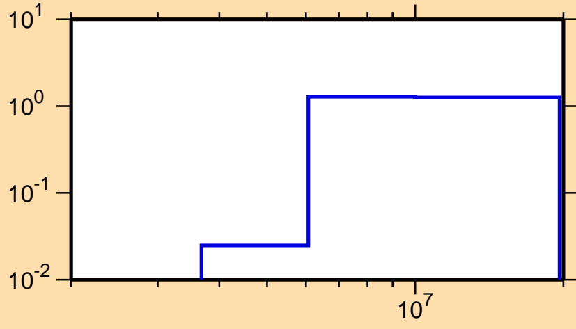
\sigma vs. E for ^{166}\text{Tb}(n,2n)
