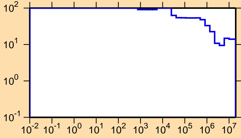
\Delta\sigma/\sigma vs. E for ^{166}\text{Tb}(n,\text{nonel.})
