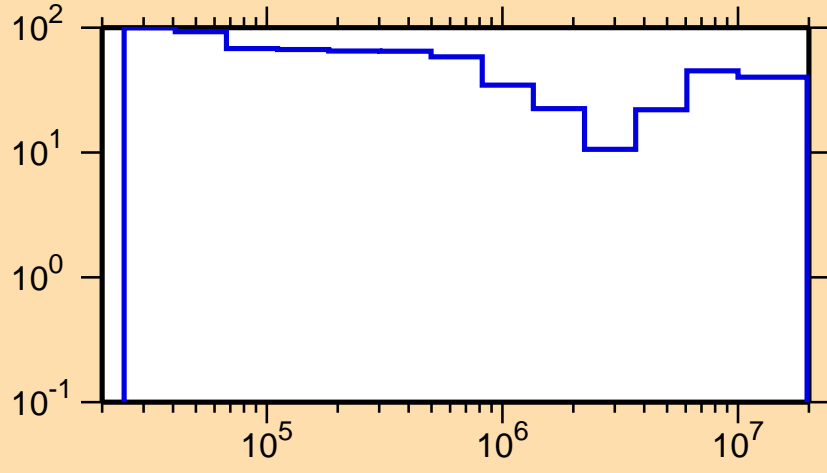
\Delta\sigma/\sigma vs. E for ^{166}\text{Tb}(n,\text{inel.})
