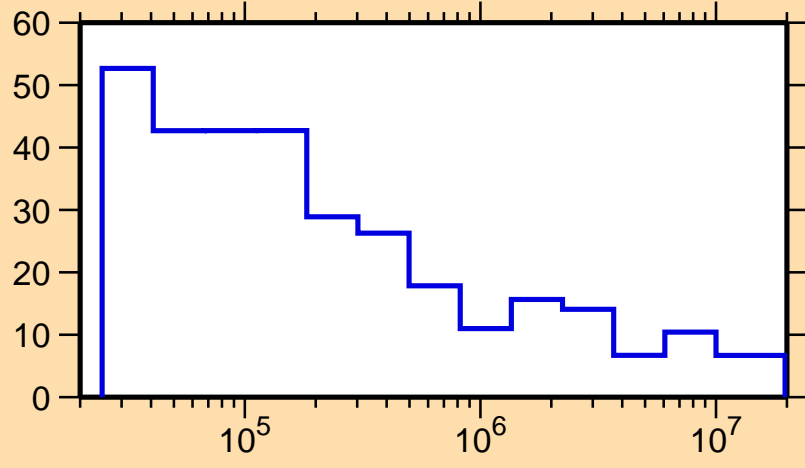
\Delta\sigma/\sigma vs. E for ^{166}\text{Tb}(n,\text{tot.})
