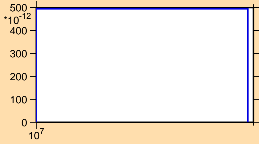
\sigma vs. E for ^{166}\text{Tb}(n,2n\alpha)
