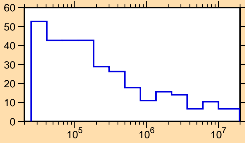
\Delta\sigma/\sigma vs. E for ^{166}\text{Tb}(n,\text{tot.})
