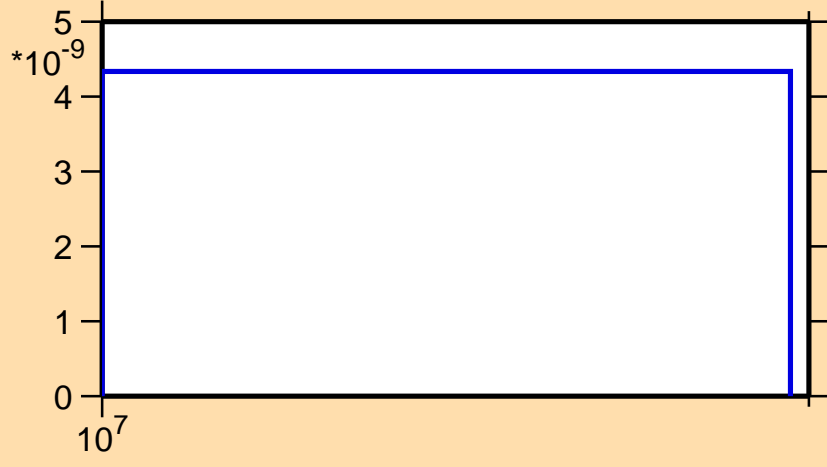
\sigma vs. E for ^{166}\text{Tb}(n,2np)
