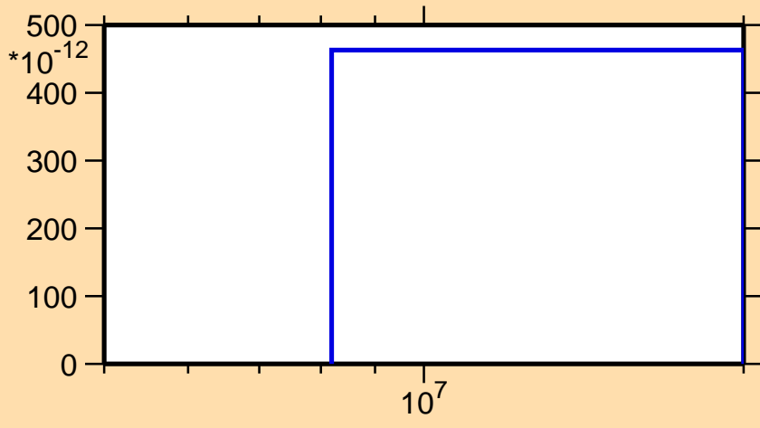
\sigma vs. E for ^{166}\text{Tb}(n,2n\alpha)
