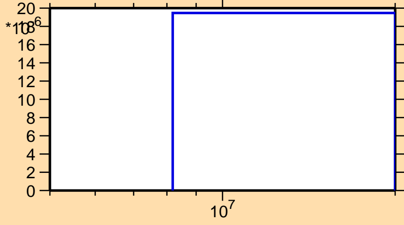
\sigma vs. E for ^{168}\text{Tb}(n,np)
