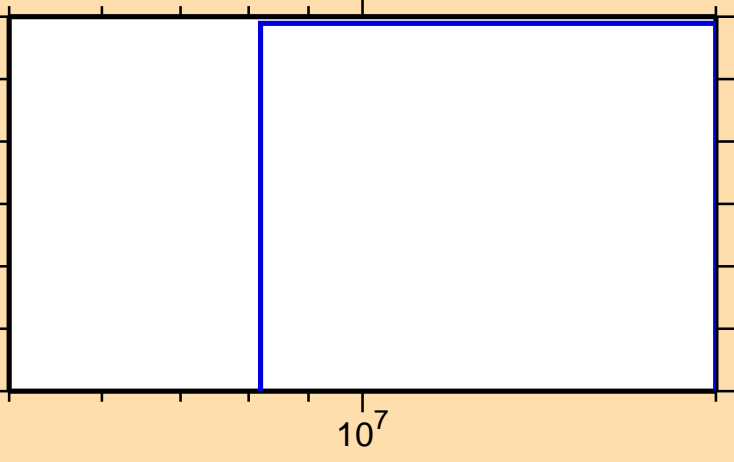
\sigma vs. E for ^{168}\text{Tb}(n,\text{nd})
