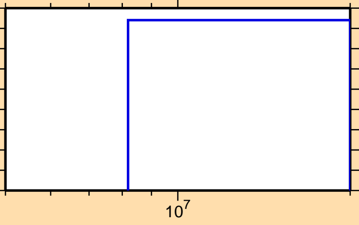
\sigma vs. E for ^{168}\text{Tb}(n,t)
