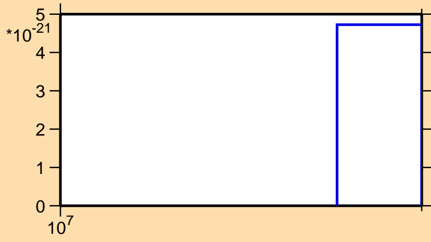
\sigma vs. E for ^{87}\text{Tc}(n,nt)
