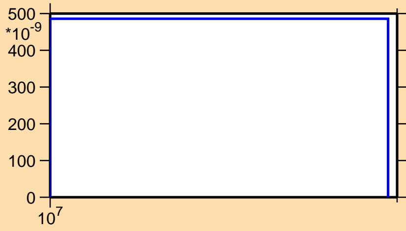
\sigma vs. E for ^{87}\text{Tc}(n,2n)
