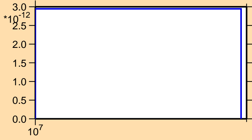
\sigma vs. E for ^{87}\text{Tc} (mt 34)
