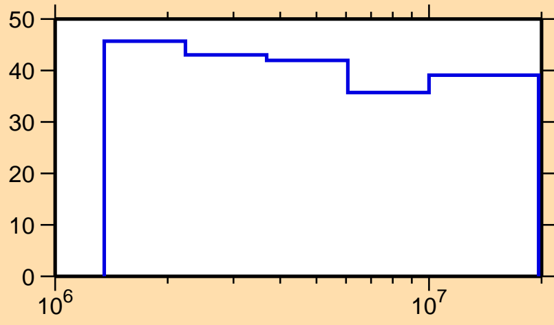
\Delta\sigma/\sigma vs. E for ^{87}\text{Tc}(n,ncont.)
