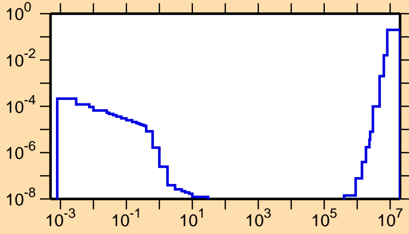
\sigma vs. E for ^{87}\text{Tc}(n,p\alpha)
