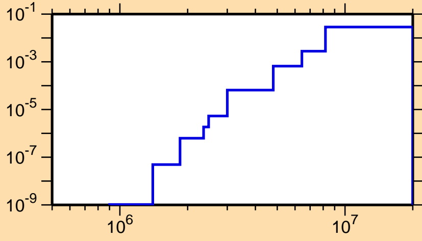
\sigma vs. E for ^{87}\text{Tc}(n,d)
