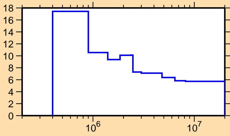
\Delta\sigma/\sigma vs. E for ^{87}\text{Tc}(n,\text{nonel.})
