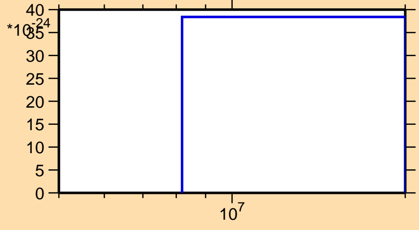
\sigma vs. E for ^{87}\text{Tc}(n,nt)
