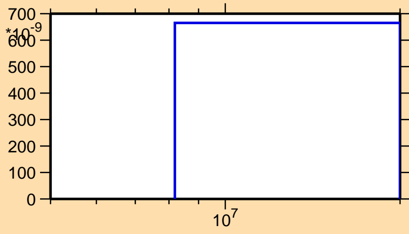
\sigma vs. E for ^{87}\text{Tc}(\text{mt } 45)
