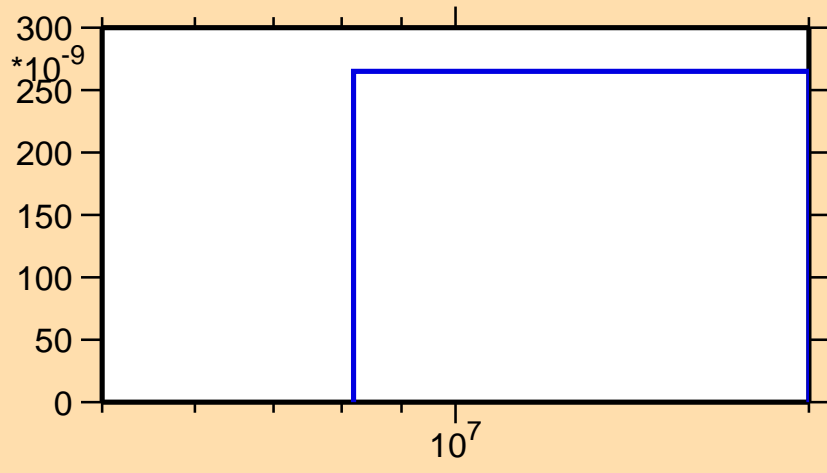
\sigma vs. E for ^{87}\text{Tc}(n,\text{pt})
