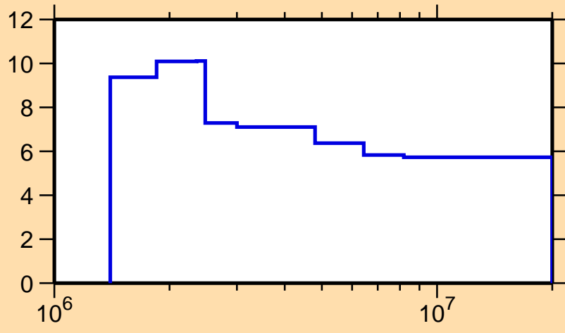
\Delta\sigma/\sigma vs. E for ^{87}\text{Tc}(n,n\text{nonel.})
