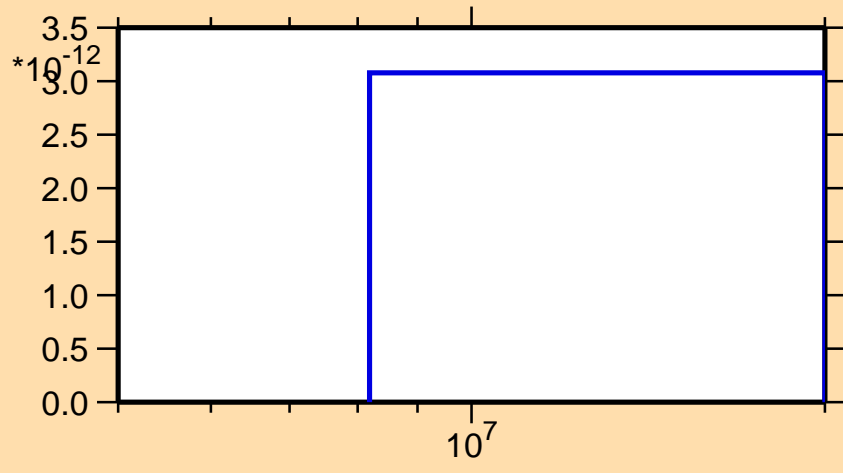
\sigma vs. E for ^{87}\text{Tc}(\text{mt } 34)
