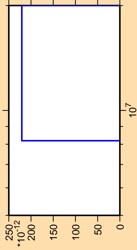
\Delta\sigma/\sigma vs. E for ^{87}\text{Tc}(n,nt)
