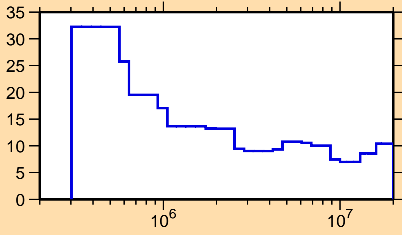
\Delta\sigma/\sigma vs. E for ^{88}\text{Tc}(n,n\text{onel.})
