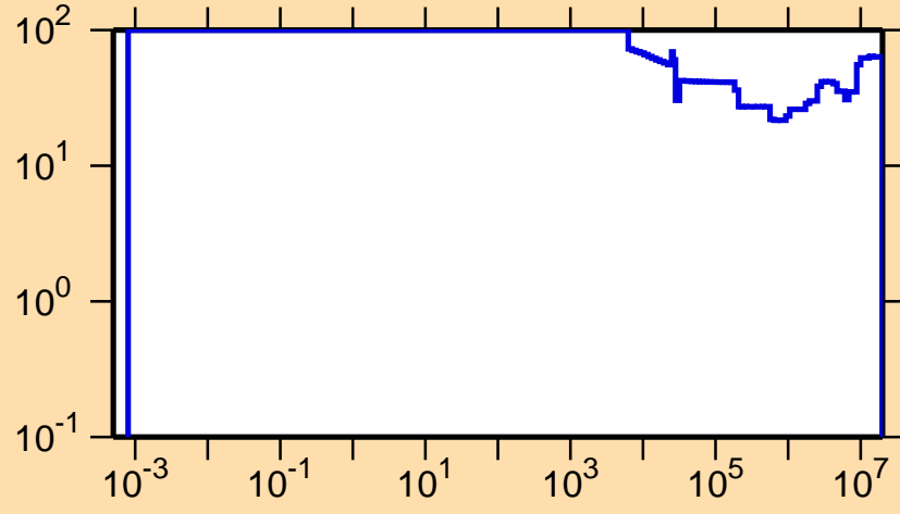
\Delta\sigma/\sigma vs. E for ^{88}\text{Tc}(n,p)
