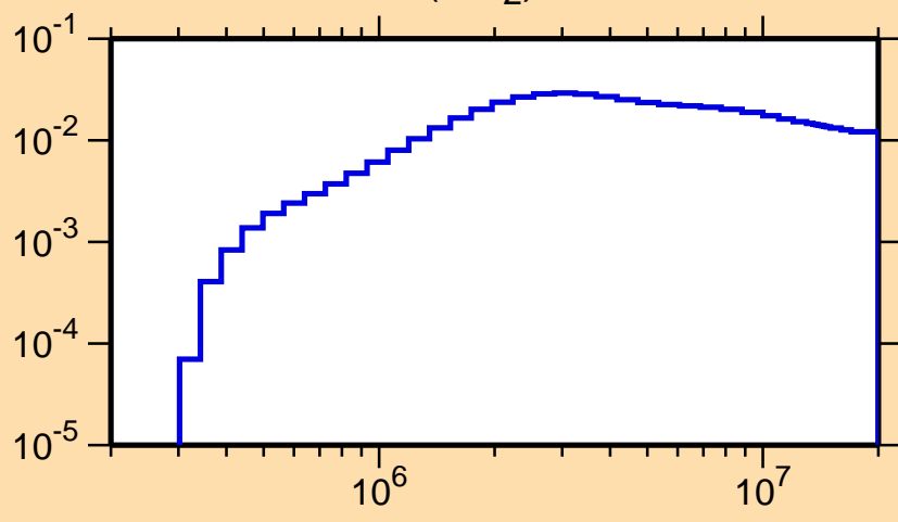
\sigma vs. E for ^{88}\text{Tc}(n,n_2)
