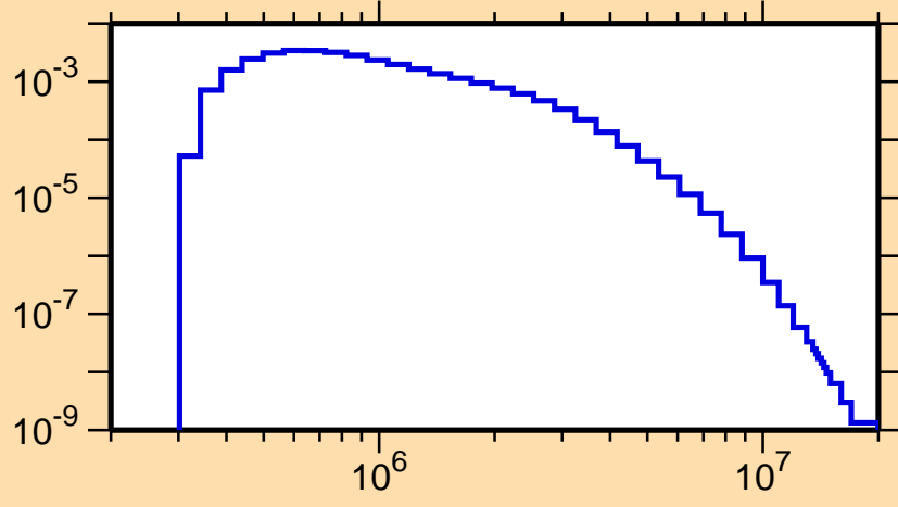
\sigma vs. E for ^{88}\text{Tc}(n,n_3)
