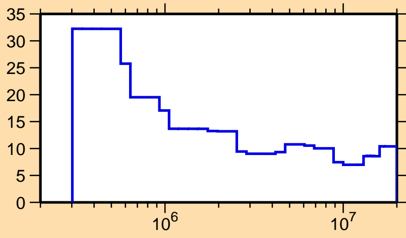
\Delta\sigma/\sigma vs. E for ^{88}\text{Tc}(n,\text{nonel.})
