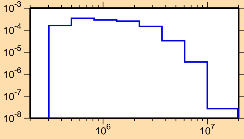
\sigma vs. E for ^{88}\text{Tc}(n,n_1)
