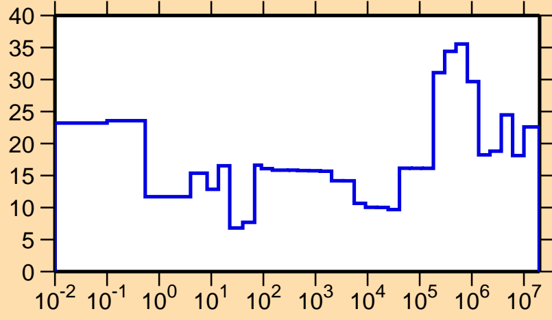
\Delta\sigma/\sigma vs. E for ^{88}\text{Tc}(n,el.)
