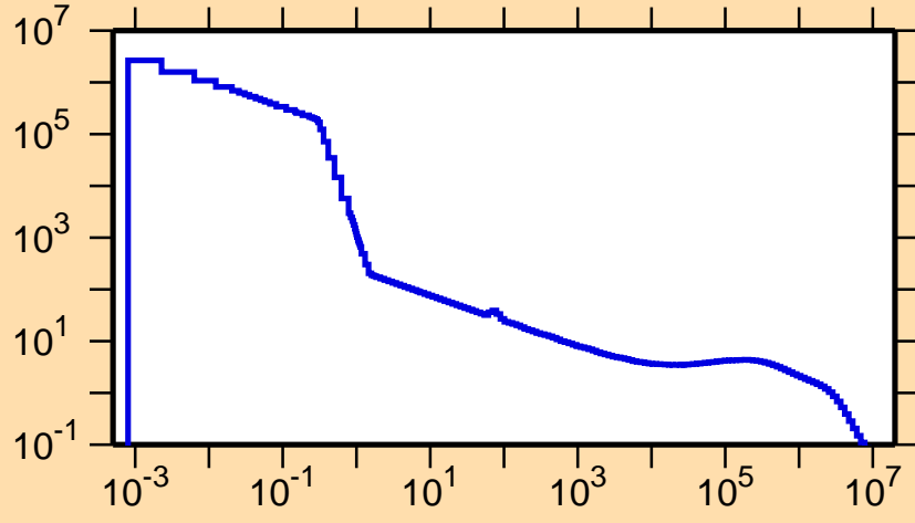
\sigma vs. E for ^{88}\text{Tc}(n,p)
