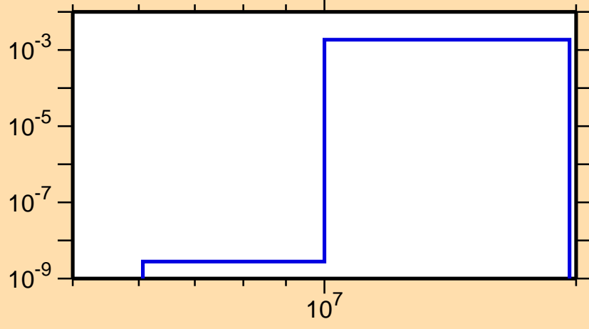
\sigma vs. E for ^{88}\text{Tc}(n,\text{pd})
