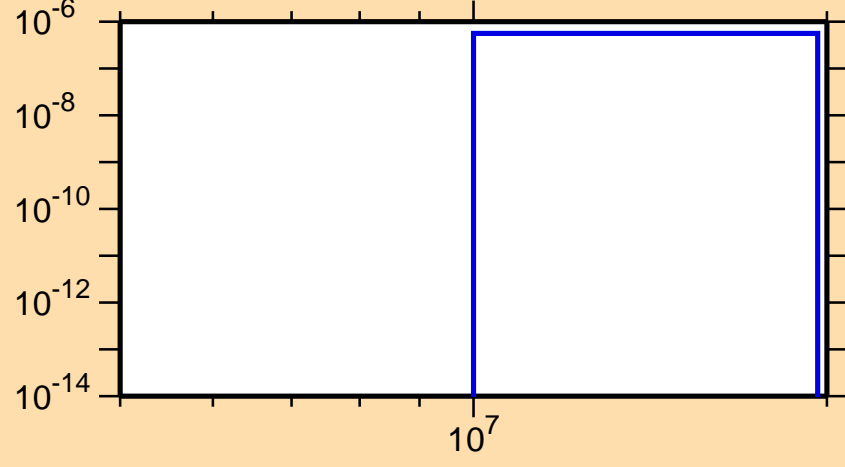
\sigma vs. E for ^{88}\text{Tc}(\text{mt } 45)
