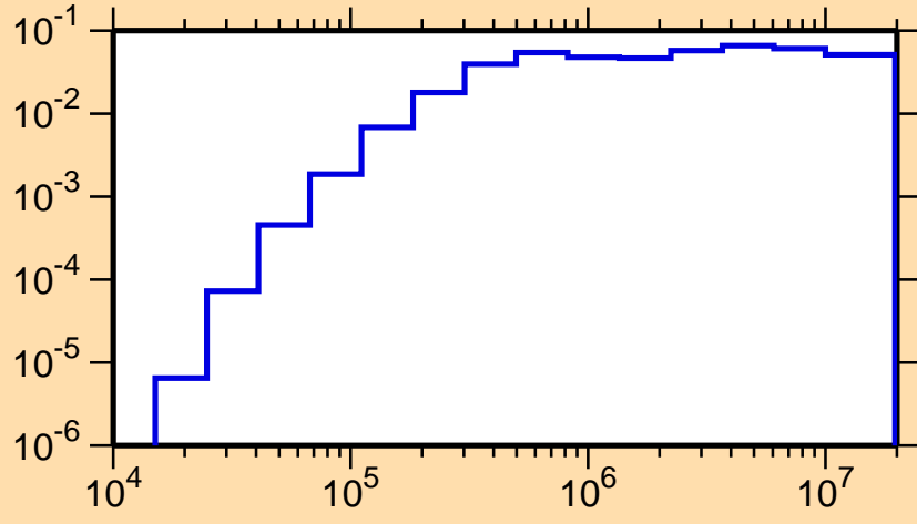
\sigma vs. E for ^{88}\text{Tc}(n,n\text{cont.})
