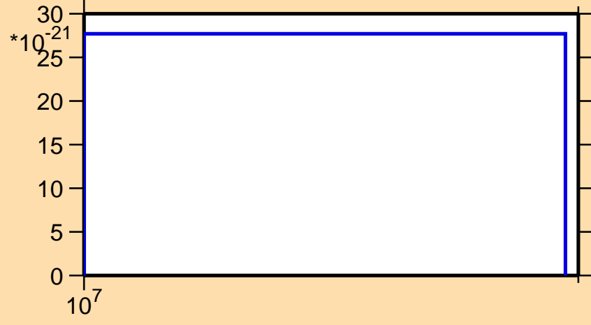
\sigma vs. E for ^{88}\text{Tc}(n,nt)
