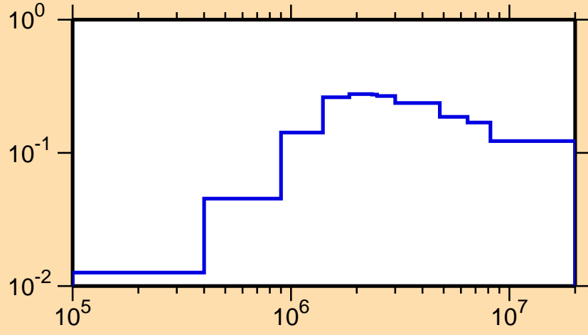
\sigma vs. E for ^{89}\text{Tc}(n,\text{inel.})
