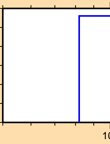
\sigma vs. E for ^{89}\text{Tc} (mt 45)
