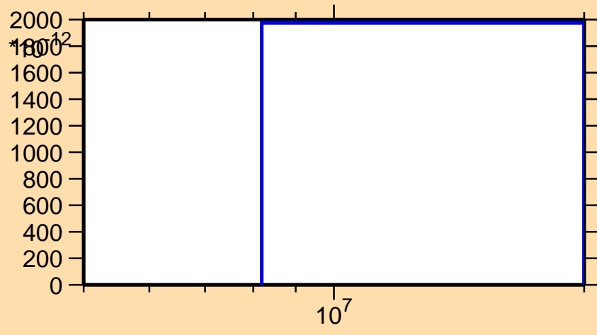
\sigma vs. E for ^{89}\text{Tc}(n,\text{pt})
