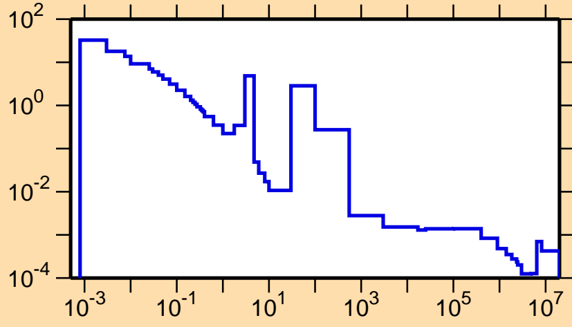
\sigma vs. E for ^{89}\text{Tc}(n,\gamma)
