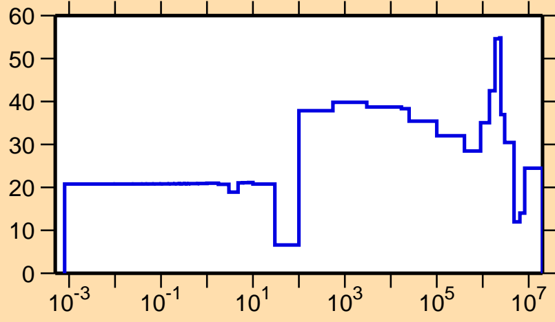
\Delta\sigma/\sigma vs. E for ^{89}\text{Tc}(n,el.)
