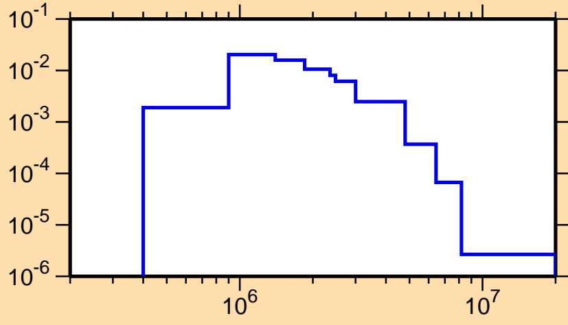
\sigma vs. E for ^{89}\text{Tc}(n,n_3)
