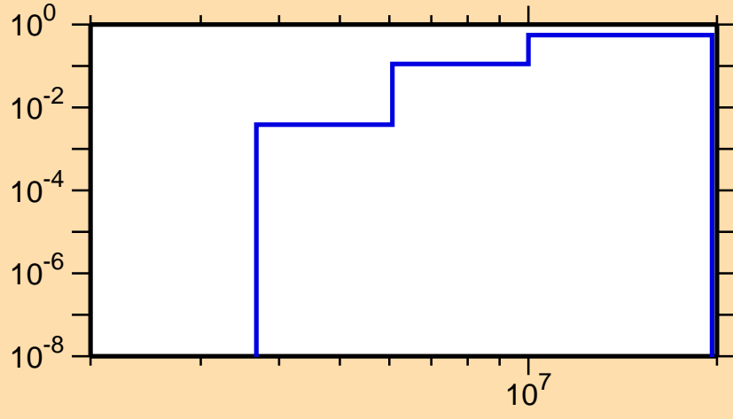
\sigma vs. E for ^{90}\text{Tc}(n,np)
