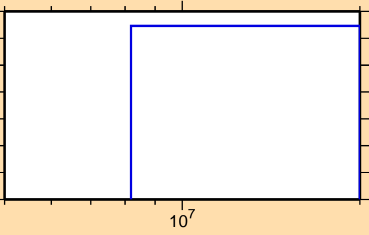
\sigma vs. E for ^{90}\text{Tc}(\text{mt } 45)
