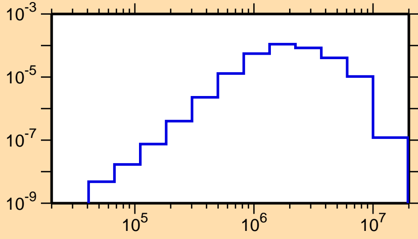
\sigma vs. E for ^{90}\text{Tc}(n,n_1)
