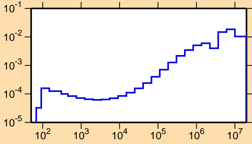
\sigma vs. E for ^{90}\text{Tc}(n,\text{inel.})
