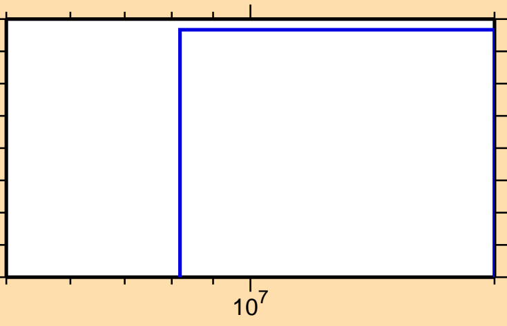
\sigma vs. E for ^{90}\text{Tc}(n,\text{nd})
