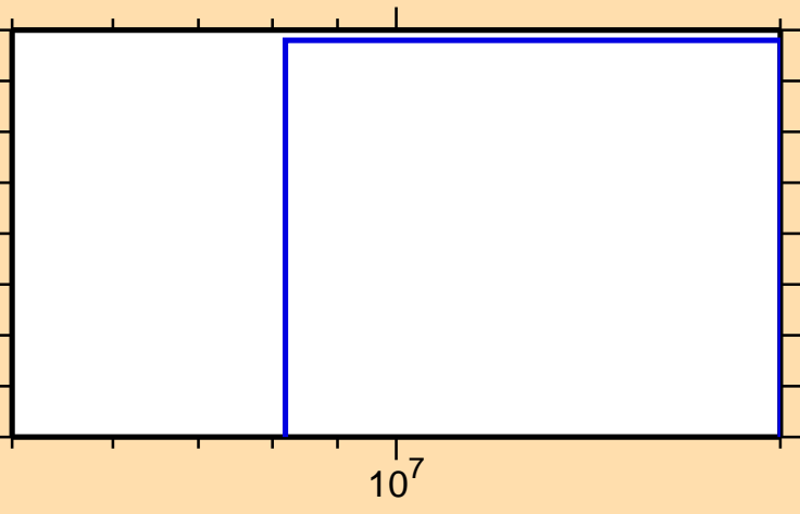
\sigma vs. E for ^{90}\text{Tc}(n,2np)
