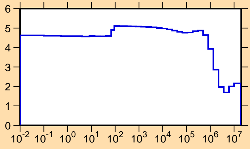
\sigma vs. E for ^{90}\text{Tc}(n,\text{el.})
