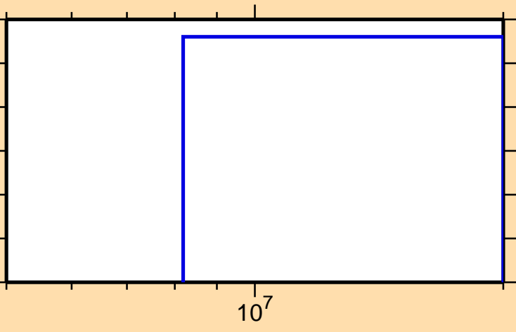
\sigma vs. E for ^{90}\text{Tc}(n,2np)
