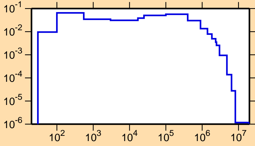
\sigma vs. E for ^{90}\text{Tc}(n,n_2)
