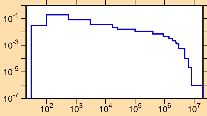
\sigma vs. E for ^{90}\text{Tc}(n,n_4)
