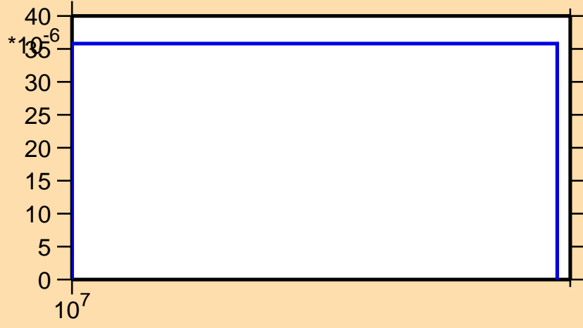
\sigma vs. E for ^{91}\text{Tc}(n,\text{pd})
