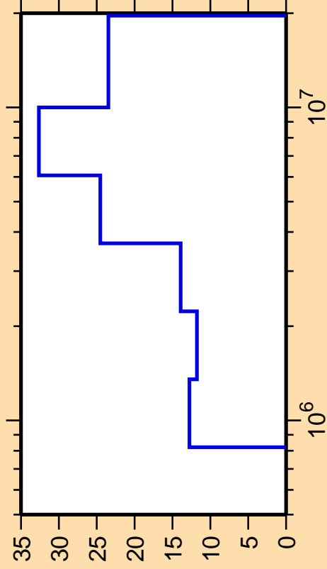
\Delta\sigma/\sigma vs. E for ^{91}\text{Tc}(n,n_4)
