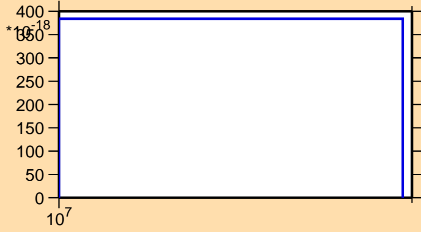
\sigma vs. E for ^{91}\text{Tc} (mt 34)
