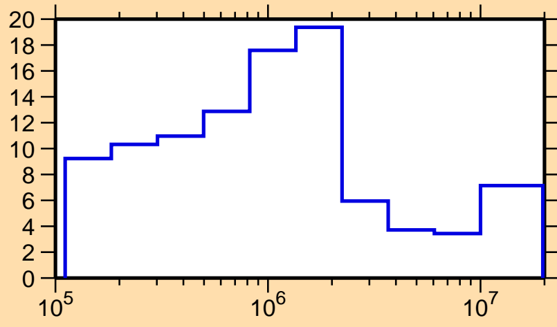
\Delta\sigma/\sigma vs. E for ^{91}\text{Tc}(n,\text{el.})
