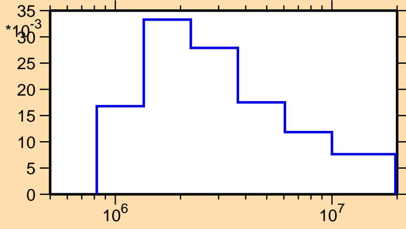
\sigma vs. E for ^{91}\text{Tc}(n,n_4)
