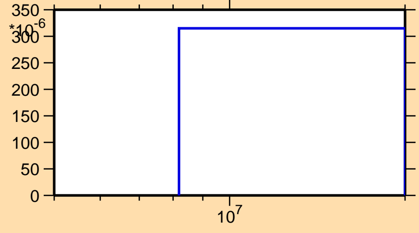
\sigma vs. E for ^{91}\text{Tc}(n,n\alpha)
