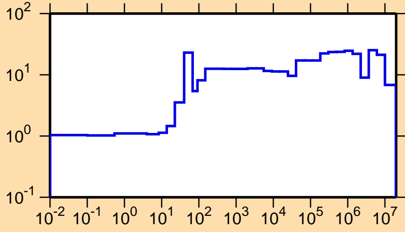
\Delta\sigma/\sigma vs. E for ^{91}\text{Tc}(n,el.)
