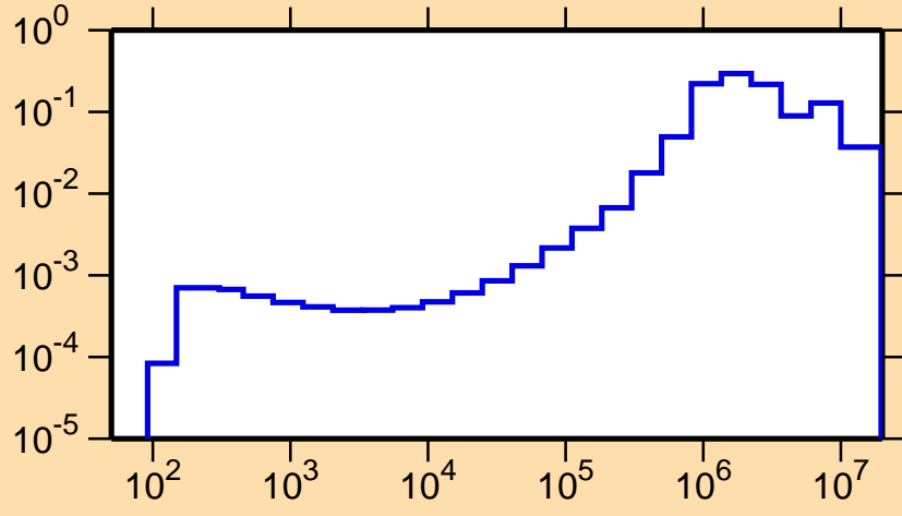
\sigma vs. E for ^{91}\text{Tc}(n,\text{inel.})
