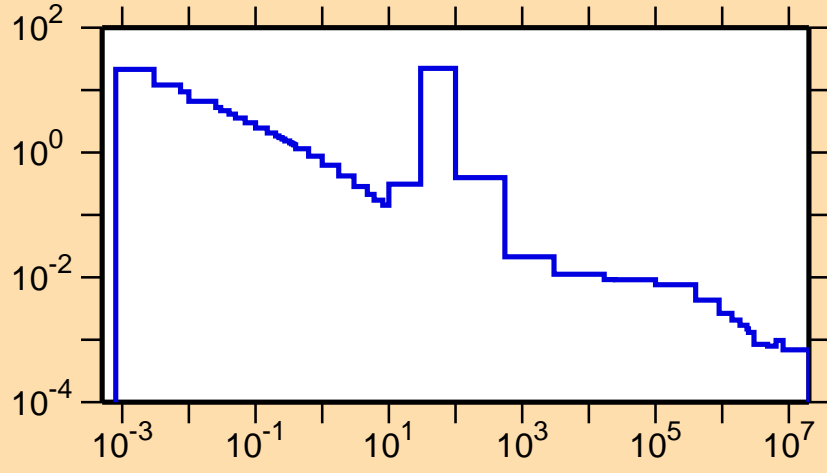
\sigma vs. E for ^{91}\text{Tc}(n,\gamma)
