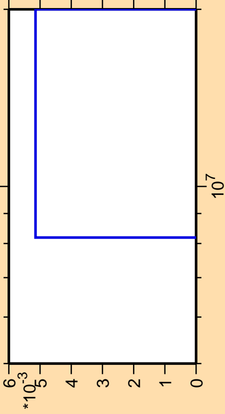
\Delta\sigma/\sigma vs. E for ^{91}\text{Tc}(\text{mt } 34)
