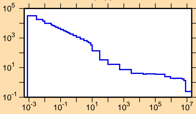
\sigma vs. E for ^{91}\text{Tc}(n,p)
