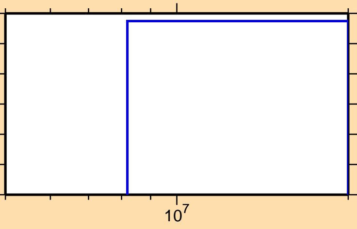
\sigma vs. E for ^{91}\text{Tc}(\text{mt } 34)
