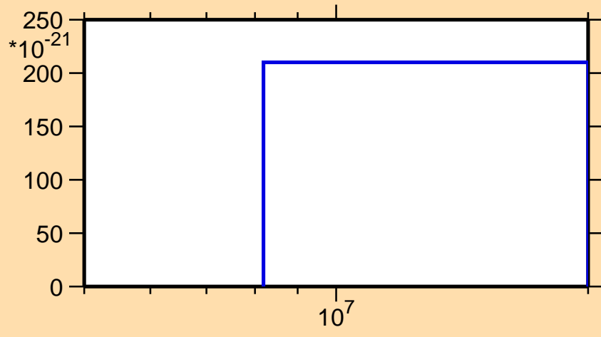
\sigma vs. E for ^{91}\text{Tc}(n,nt)
