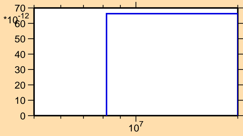
\sigma vs. E for ^{91}\text{Tc}(\text{mt117})
