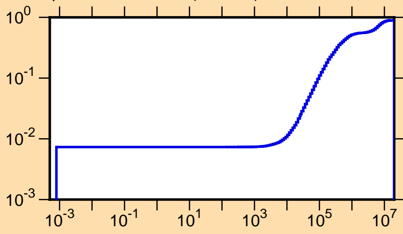
\mu vs. E for ^{92}\text{Tc}(\text{mt251})
