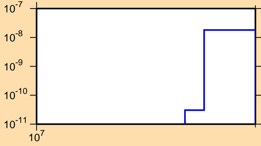
\sigma vs. E for ^{92}\text{Tc} (mt 45)
