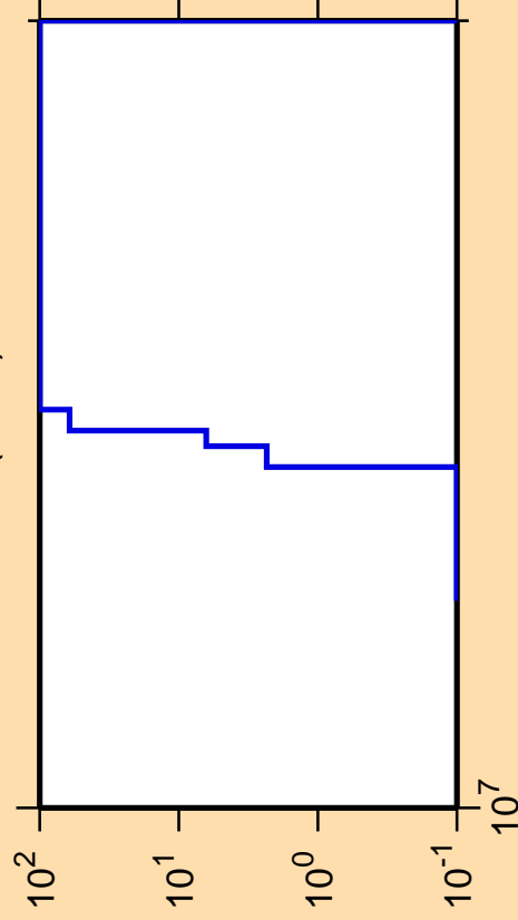
\Delta\sigma/\sigma vs. E for ^{92}\text{Tc}(n,nd)
