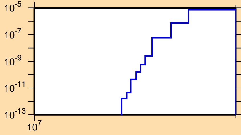
\sigma vs. E for ^{92}\text{Tc}(n,nd)
