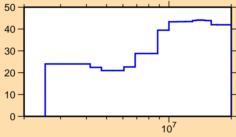
\Delta\sigma/\sigma vs. E for ^{92}\text{Tc}(n,ncont.)
