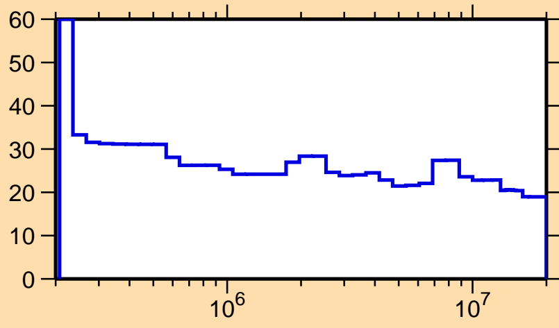
\Delta\sigma/\sigma vs. E for ^{92}\text{Tc}(n,n_1)
