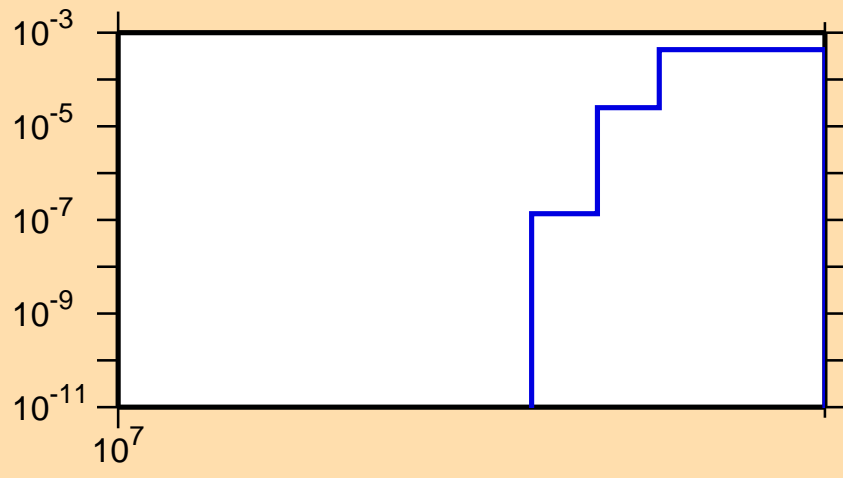
\sigma vs. E for ^{92}\text{Tc}(n,2np)
