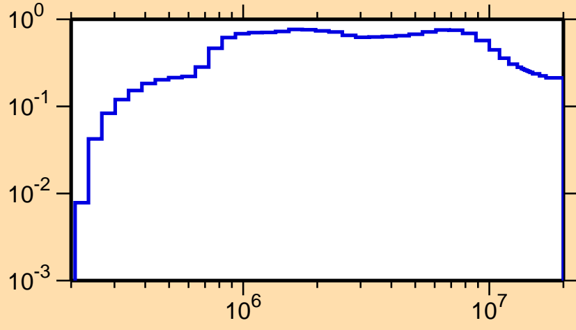
\sigma vs. E for ^{92}\text{Tc}(n,\text{inel.})
