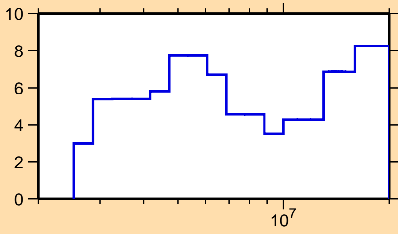
\Delta\sigma/\sigma vs. E for ^{92}\text{Tc}(n, el.)
