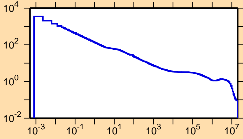
\sigma vs. E for ^{92}\text{Tc}(n,p)
