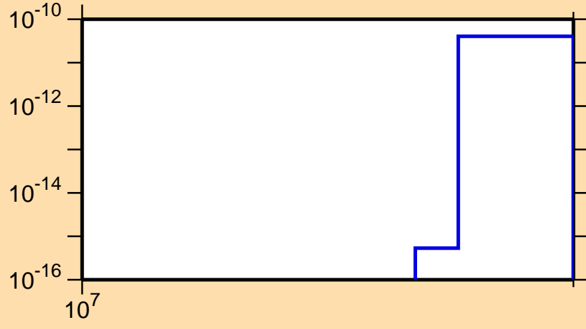
\sigma vs. E for ^{92}\text{Tc} (mt 34)
