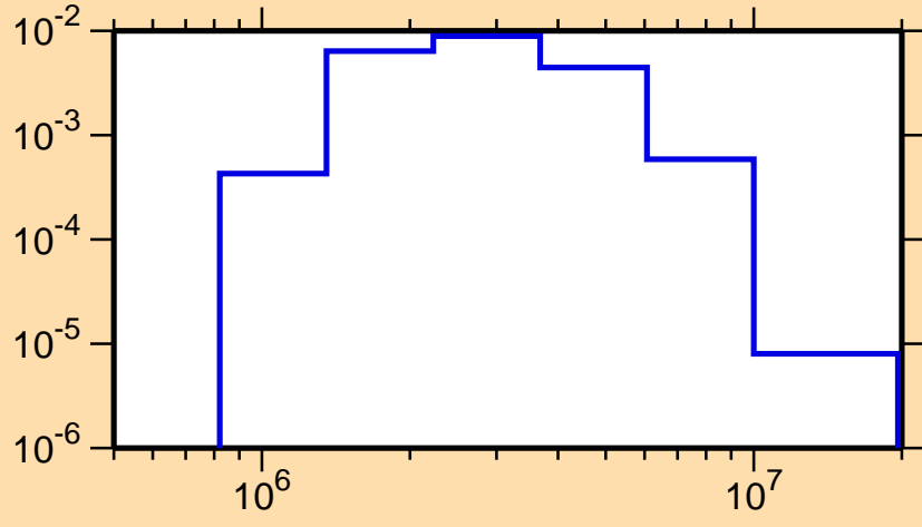
\sigma vs. E for ^{93}\text{Tc}(n,n_3)
