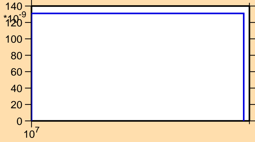
\sigma vs. E for ^{93}\text{Tc}(n,2np)
