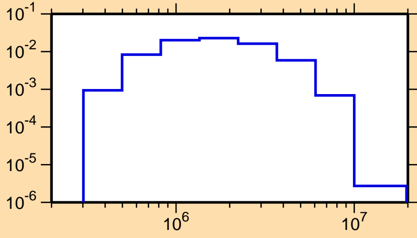
\sigma vs. E for ^{93}\text{Tc}(n,n_1)
