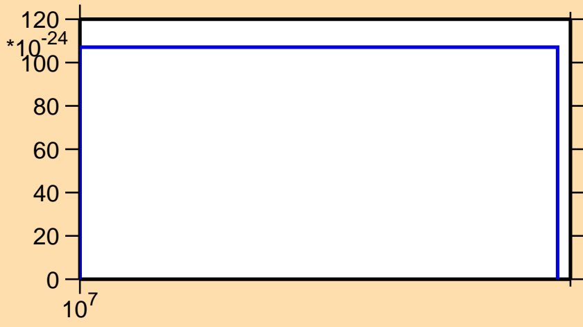
\sigma vs. E for ^{93}\text{Tc}(n,2n\alpha)
