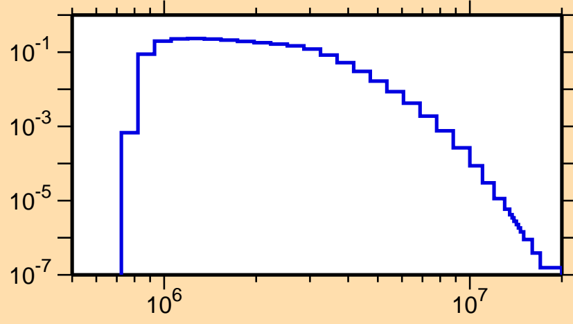
\sigma vs. E for ^{93}\text{Tc}(n,n_4)
