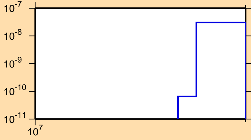
\sigma vs. E for ^{93}\text{Tc} (mt 45)
