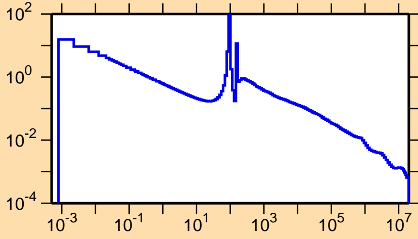
\sigma vs. E for ^{93}\text{Tc}(n,\gamma)
