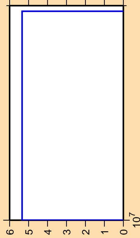
\Delta\sigma/\sigma vs. E for ^{93}\text{Tc}(\text{mt117})
