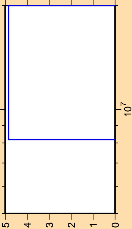
\Delta\sigma/\sigma vs. E for ^{93}\text{Tc}(\text{mt117})
