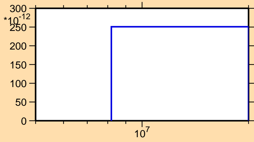
\sigma vs. E for ^{93}\text{Tc}(\text{mt } 45)
