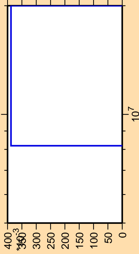
\Delta\sigma/\sigma vs. E for ^{93}\text{Tc}(n,\text{pt})
