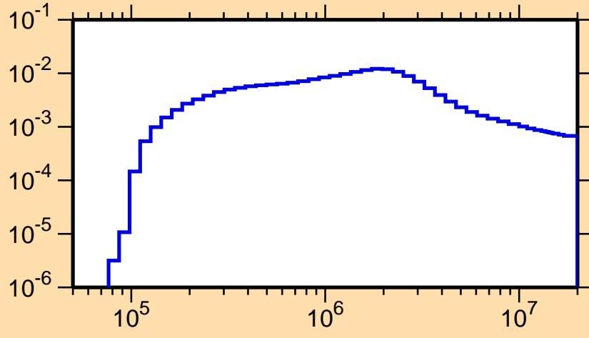
\sigma vs. E for ^{94}\text{Tc}(n,n_1)
