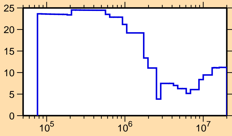
\Delta\sigma/\sigma vs. E for ^{94}\text{Tc}(n,\text{tot.})
