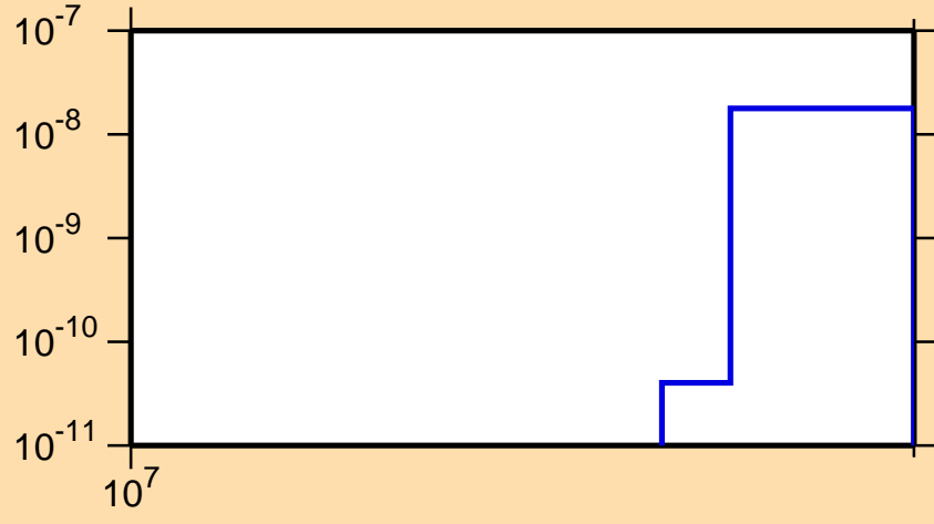
\sigma vs. E for ^{94}\text{Tc} (mt 45)
