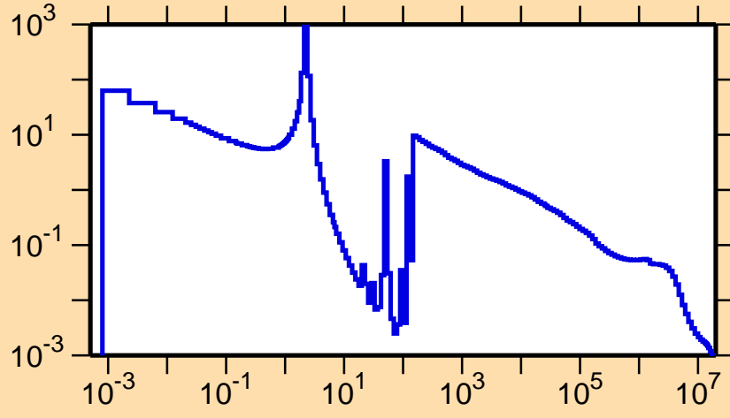
\sigma vs. E for ^{94}\text{Tc}(n,\gamma)
