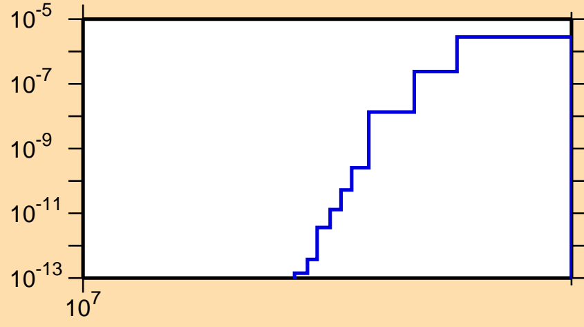
\sigma vs. E for ^{94}\text{Tc}(n,\text{pd})
