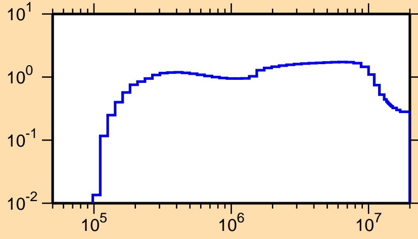
\sigma vs. E for ^{94}\text{Tc}(n,\text{inel.})
