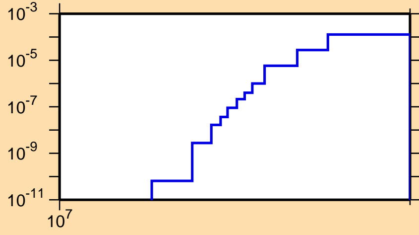
\sigma vs. E for ^{94}\text{Tc}(n,\text{nd})
