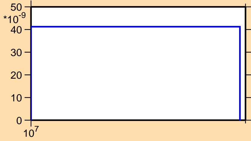
\sigma vs. E for ^{94}\text{Tc}(n,pd)
