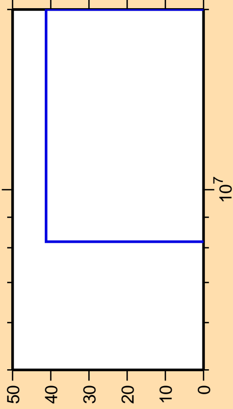
\Delta\sigma/\sigma vs. E for ^{94}\text{Tc}(\text{mt } 34)
