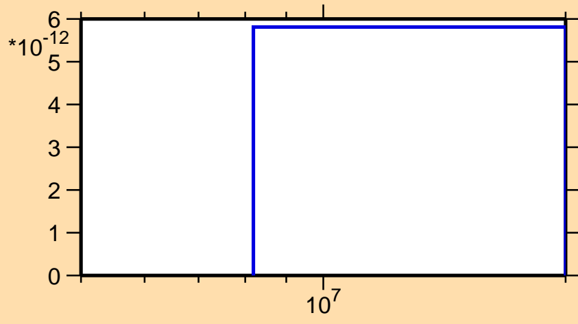
\sigma vs. E for ^{94}\text{Tc}(\text{mt } 34)
