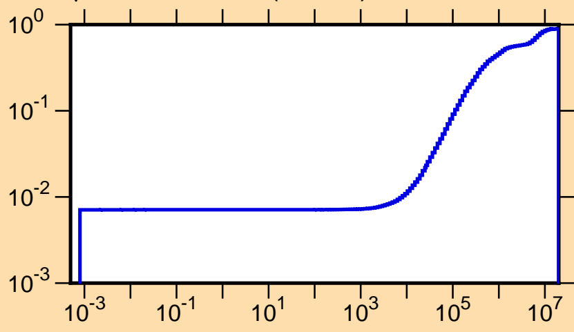
\mu vs. E for ^{95}\text{Tc}(\text{mt251})
