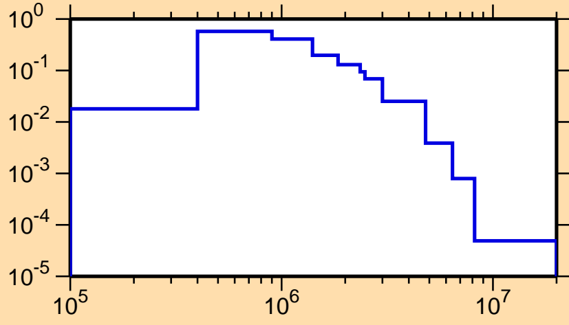
\sigma vs. E for ^{95}\text{Tc}(n,n_2)
