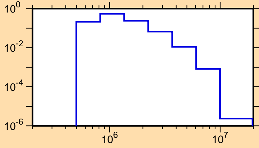
\sigma vs. E for ^{95}\text{Tc}(n,n_4)
