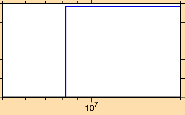
\sigma vs. E for ^{95}\text{Tc}(n,3n)
