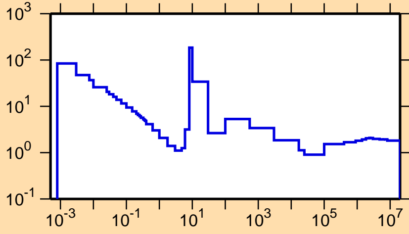
\sigma vs. E for ^{96}\text{Tc}(n,\text{nonel.})
