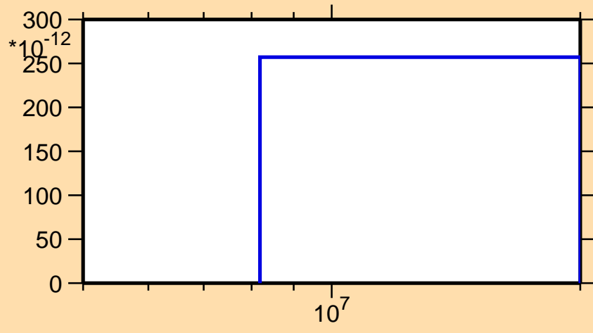
\sigma vs. E for ^{96}\text{Tc}(\text{mt } 45)
