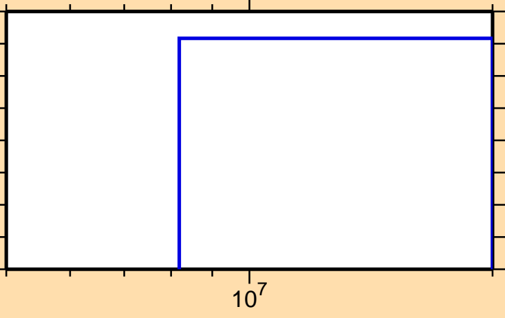
\sigma vs. E for ^{97}\text{Tc}(n,3n)
